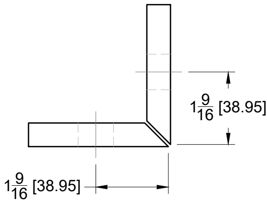
45° Mitered Glass Option (Glass Thickness 3/8 to 1/2 - 9.5 mm to 12.7 mm) (Gap 1/16 - 1.5 mm)
