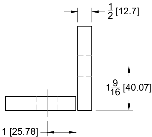
(Glass Thickness 1/2 - 12.7 mm) (Gap 1/16 - 1.5 mm)
