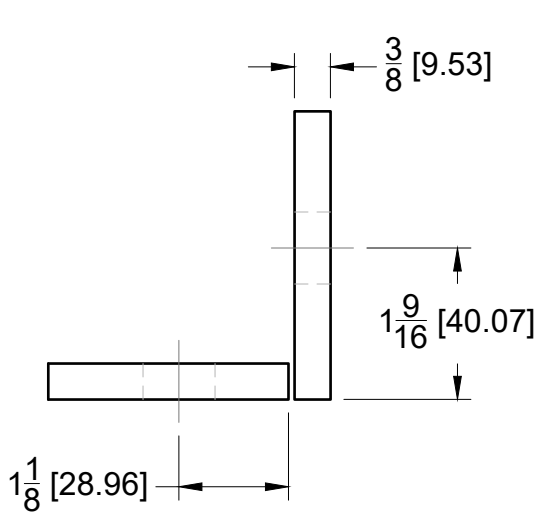
Square Cut Glass Option (Glass Thickness 3/8 - 9.5 mm) (Gap 1/16 - 1.5 mm)
