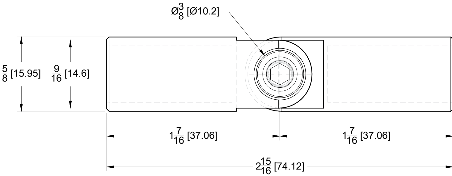
FRONT VIEW
