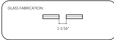
DETAIL B
